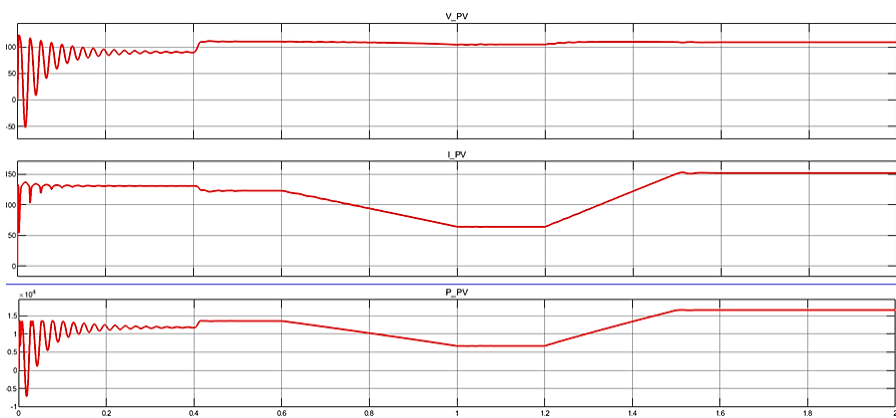
Figure 16: Voltage, current, and power output from the PV array under variable test conditions using the INC algorithm
