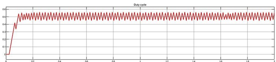
Figure 14: The duty cycle of P&O Algorithm
